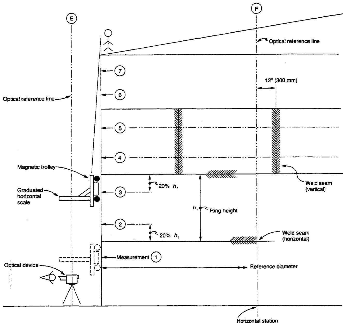
Figure 2—Tank Elevation
