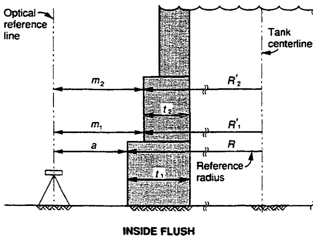
Figure 3—Optical Reference Line Method: Determination of Internal Radius (External Measurement)
